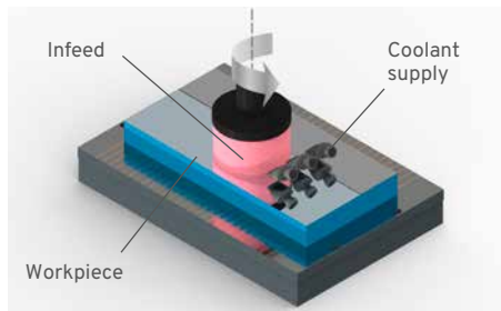
Vertical spindle, reciprocating table
