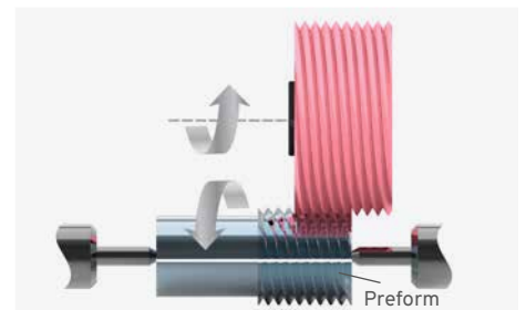
Plunge-cut thread grinding
