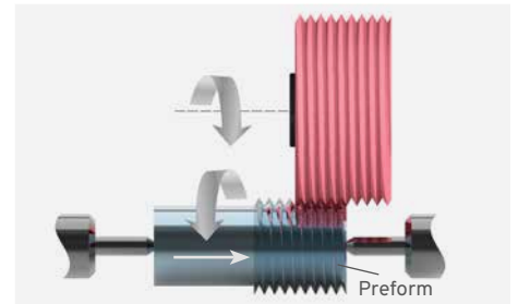
Transverse thread grinding
