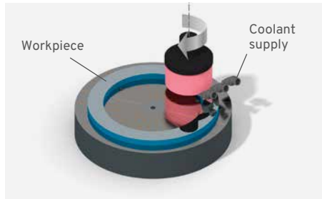
Vertical spindle, rotary table
