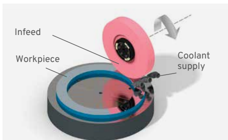
Horizontal spindle, rotary table
