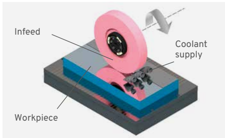
Horizontal spindle, reciprocating table
